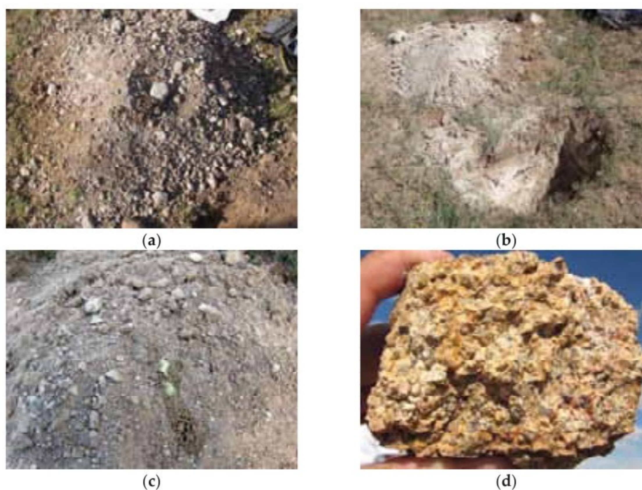
Figure 6. (a) WK183 light grayish-brown carbonaceous conglomerate with loose pebbles; (b) WK184 brownish-gray fine-grained sand, whitish-gray siltstone and dark to light gray siltstone; (c) WK161 brown sand with granite fragments clasts; yellow in the center is the reaction of nitric acid and ammonium molybdate with phosphorus in the sample; (d) WK157 coarse-grained granite, Late Triassic—Early Jurassic age.
