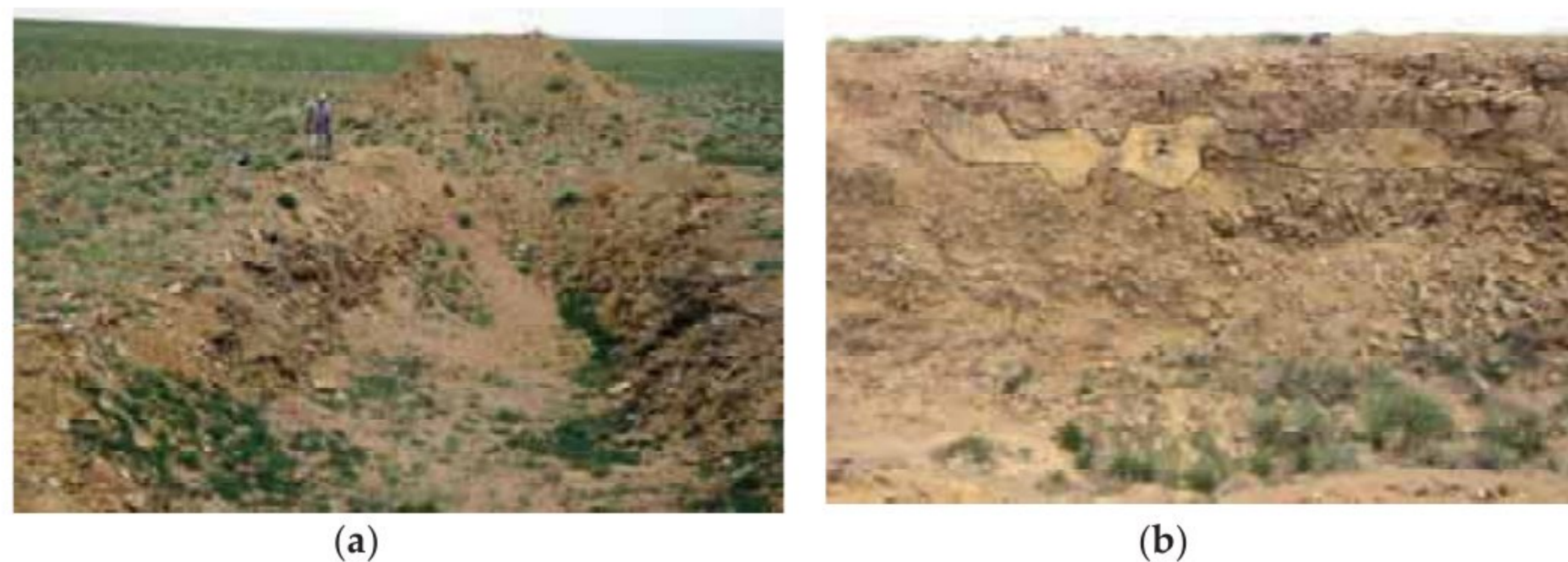
Figure 8. (a) Old Russian trench (dug in 1980). General overview. Conglomerate and sandstone trending to SE; (b) Historic exploration trench, the picture is of NE wall of the trench, length of the section marked with a black line is approximately 6 m. 1. Dark gray sandstone, 2. Conglomerate and coarse-grained sandstone bearing phosphate, measured with RS125 spectrometer: U—93 ppm, Th—75 ppm, K—0.8%, radioactivity was 720 cps and 3. Gray phosphatic sandstone.
