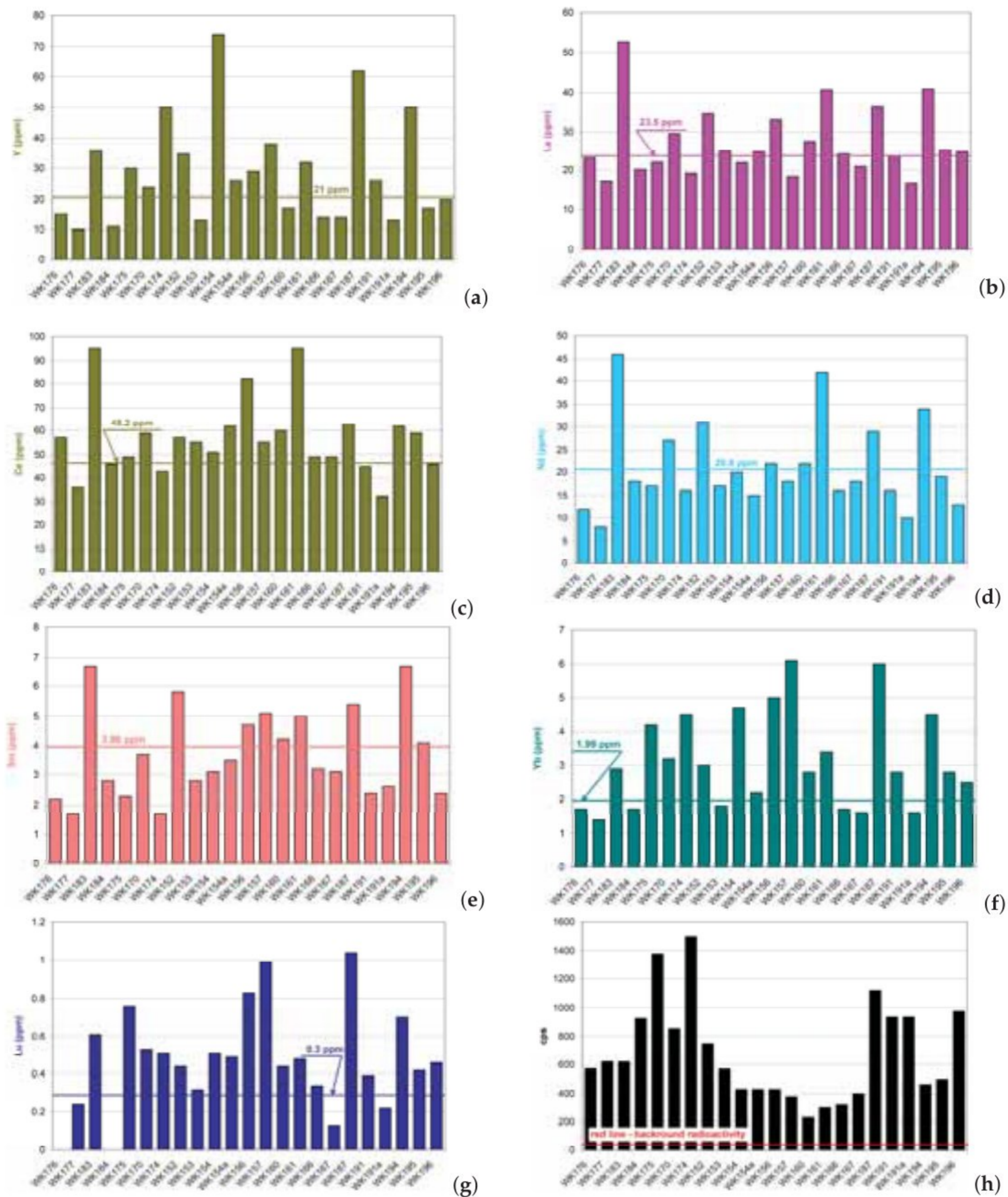
Figure 5. Graphics of grades (a) yttrium—Y, (b) lanthanum—La, (c) cerium—Ce, (d) neodymium—Nd, (e) samarium—Sm, (f) ytterbium—Yb, (g) lutetium—Lu and (h) radioactivity in counts/sec (cps).
