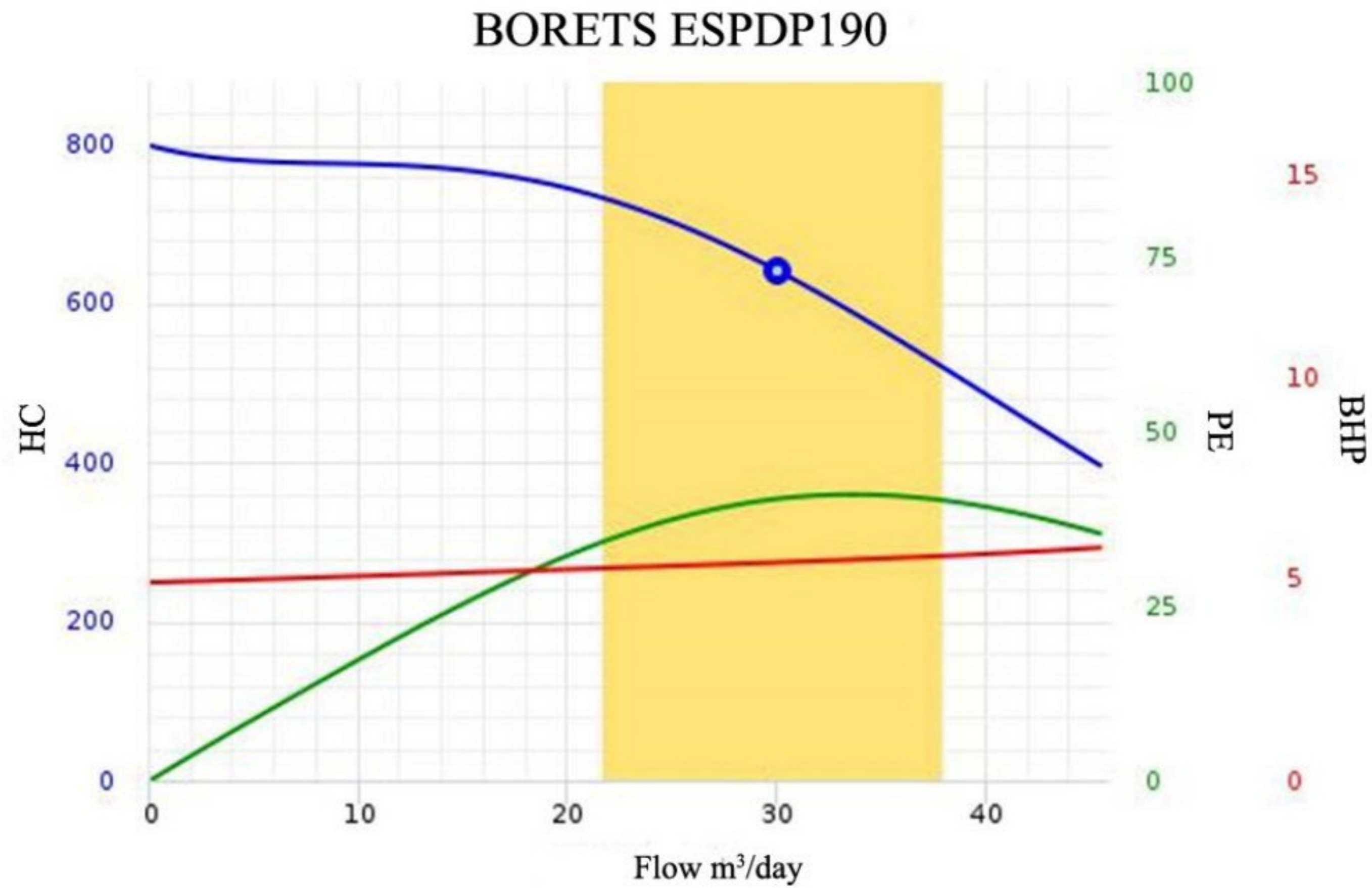
Figure 4 The ESP pump performance curve (“Pengtools.com”)
