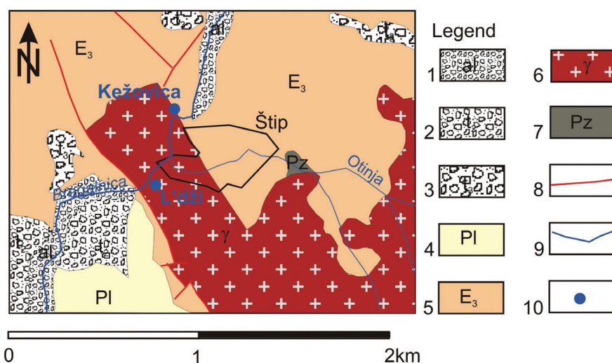
Fig. 1. Geological map of the extended area of the spa town of Kežovica and the L'dži locality. Legend: 1, alluvium (gravel, sand and clay); 2, lower terrace (conglomerate, clay, marl and sandstone); 3, upper terrace (conglomerate, clay, marl and sandstone); 4, Pliocene sediments; 5, upper Eocene conglomerate, marl, sandstone, and flysch; 6, granite massif; 7, gneiss and mica schist of Pre-Mesozoic age; 8, fault; 9, river; 10, thermomineral spring.
