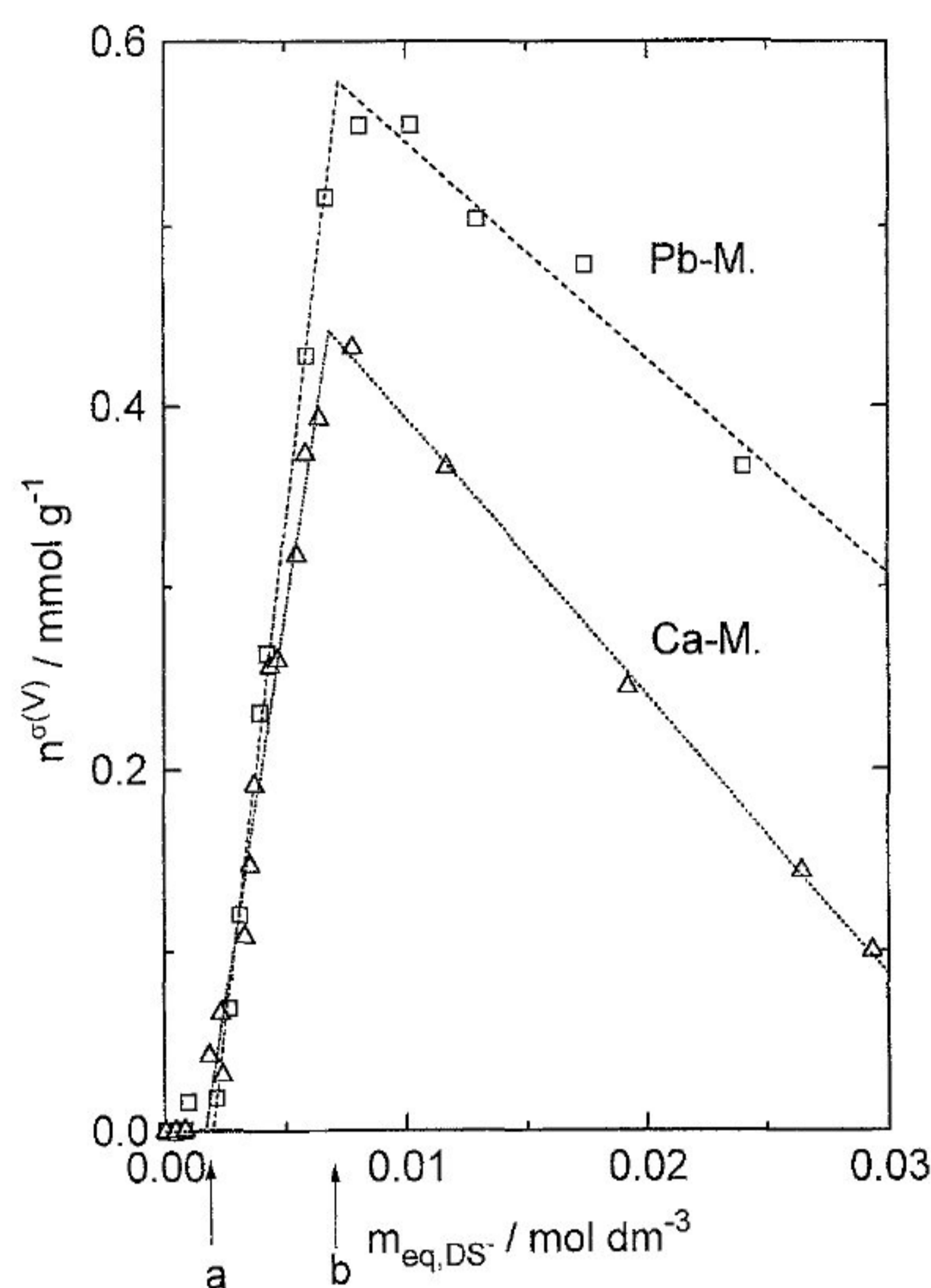
Fig. 2 Specific surface excess n_{\text{DS}}^{\sigma(V)} , Eq. (6), for Ca- and Pb-montmorillonite at a concentration of 15 \text{ g} \cdot \text{dm}^{-3} . “ a ” and “ b ” denote the beginning of the precipitation and the solubilization, respectively
