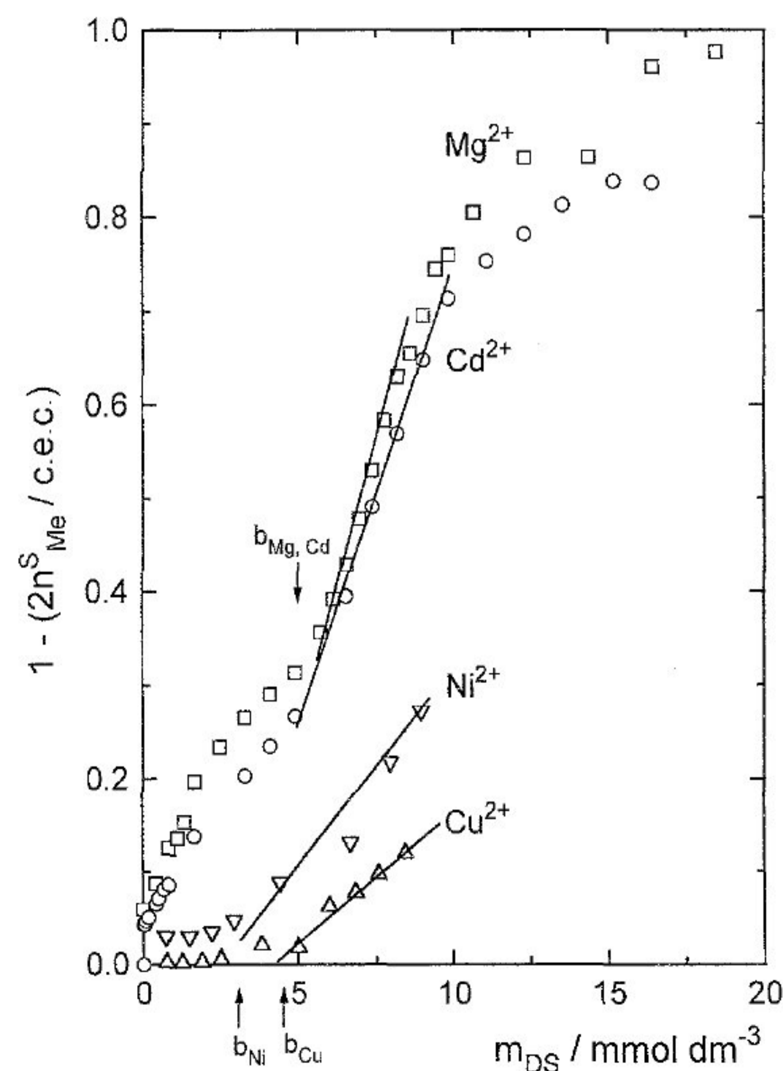
Fig. 7 Mobilization of \text{Mg}^{2+} , \text{Cd}^{2+} , \text{Ni}^{2+} and \text{Cu}^{2+} by \text{DS}^- . ( 1 - 2n_{\text{M}}^{\text{S}} / \text{c.e.c.} ) is the normalized amount of the metal ions desorbed into the bulk phase. The lines indicate the enhanced mobilization above the CMC "a": beginning of the precipitation; "b": beginning of the mobilization (dispersion concentrations: 0.5 \text{ g dm}^{-3} for Mg- and Cd-montmorillonite and 9.5 \text{ g dm}^{-3} for Ni- and Cu-montmorillonite)
