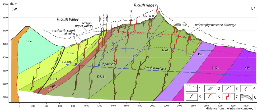
Figure 5 : A quasi-3D conceptual model of the contemporary Tukush karst hydrogeological system.
