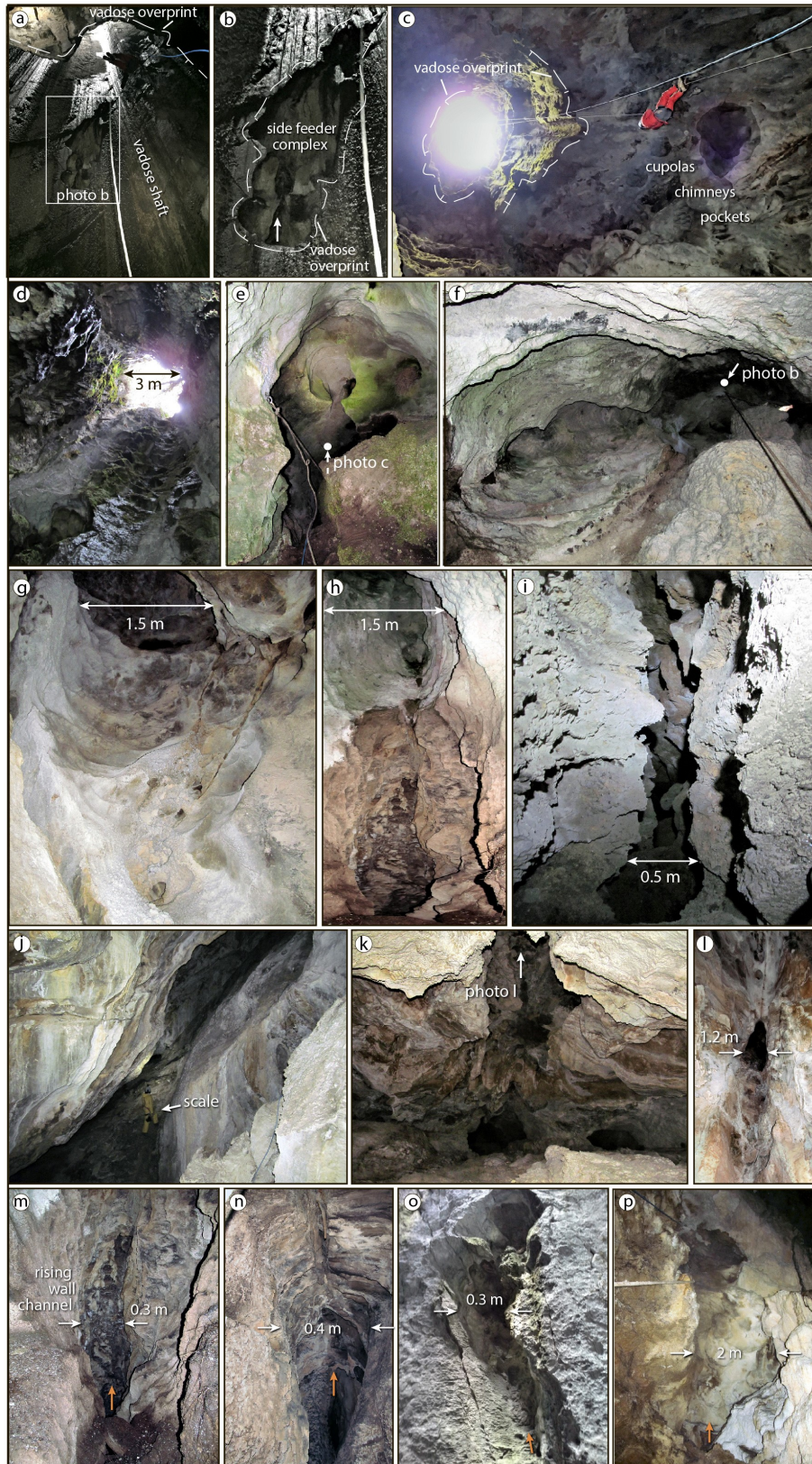
Figure 4: Morphological features of caves in the Tucush area. a-c – the overprinting of vadoso dissolution surfaces onto hypogene morphs; d – hypogene shaft open to the surface; e – the top of the internal shaft viewed from above; f and h – features at the tops of internal shafts, viewed from below (f is the same shaft shown in e); i – rift-like passage; j-l – inclined, bedding-controlled chamber (j – strike-parallel view; k – up-dip view where the arrow points to a rising chimney/shaft shown in photo l as viewed from below); m-p – side feeders in the shaft walls. Caves: a, b, i – CTU09; c – CTU165, g, h, m, n – CTU162; j, k, l – CTU89; o, p – CTU164.
