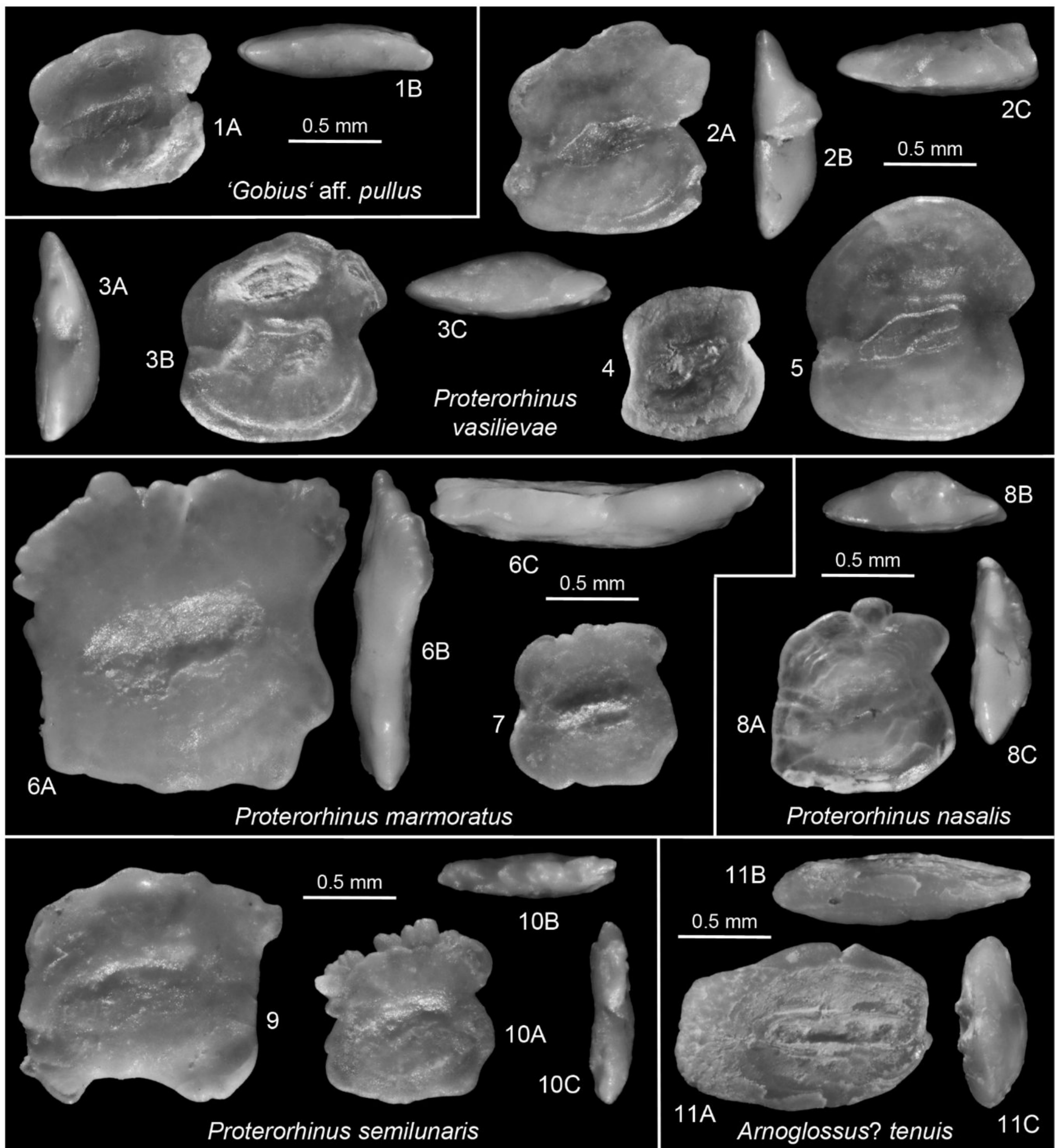
Fig. 8 1 “ Gobius ” aff. pullus Kramberger-Gorjanovic 1883. IGOTBAB1/11, Barajevo-1, 65–70 m, late Badenian, ventral view (1). 2–5 Proterorhinus vasilievae n.sp. 2 Holotype, IGOTBAB1/12, Barajevo-1, 60–65 m, late Badenian, posterior view (2B), dorsal view (2C); 3 (mirrored): Paratype, IGOTBAB1/13, Barajevo-1, 80–85 m, late Badenian, posterior view (3A), dorsal view (3C); 4 (mirrored): Paratype, IGOTBAB3/4, Barajevo-3, 61–64 m, Sarmatian, early Volhynian; 5 (mirrored): Paratype, IGOTBAB1/17, Barajevo-1, 60–65 m, late Badenian. 6–7 Proterorhinus marmoratus (Pallas 1814). Recent; 6 ZMMU P.21488, Aegean Sea, SL = 62 mm; 7:
